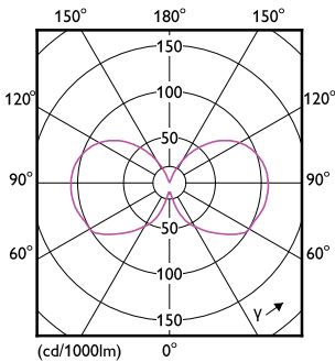
LEDCapsule CorePro 3,2W G9 830-LDD
