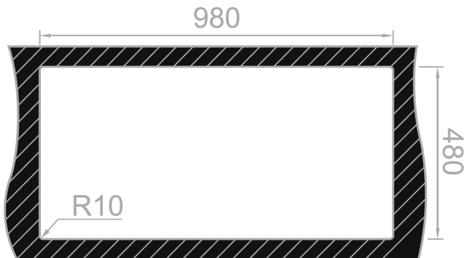
Inset Installation
