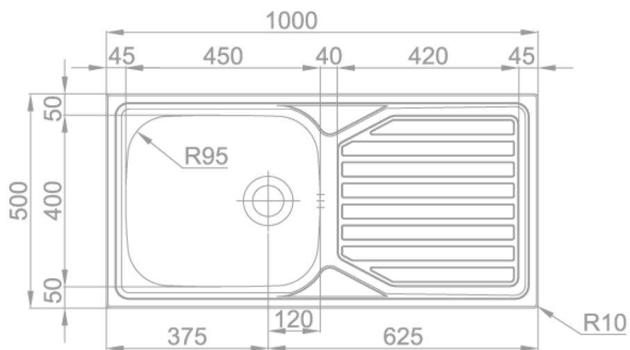
Technical Drawing
